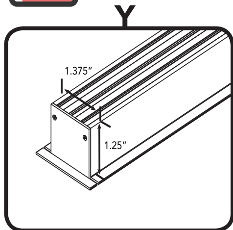
Direct Screw Installation
