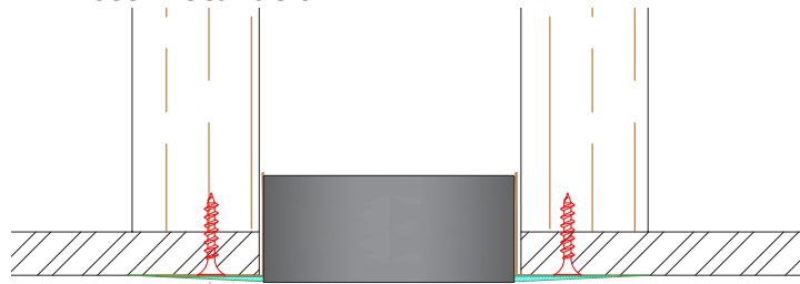
Trimless Installation
